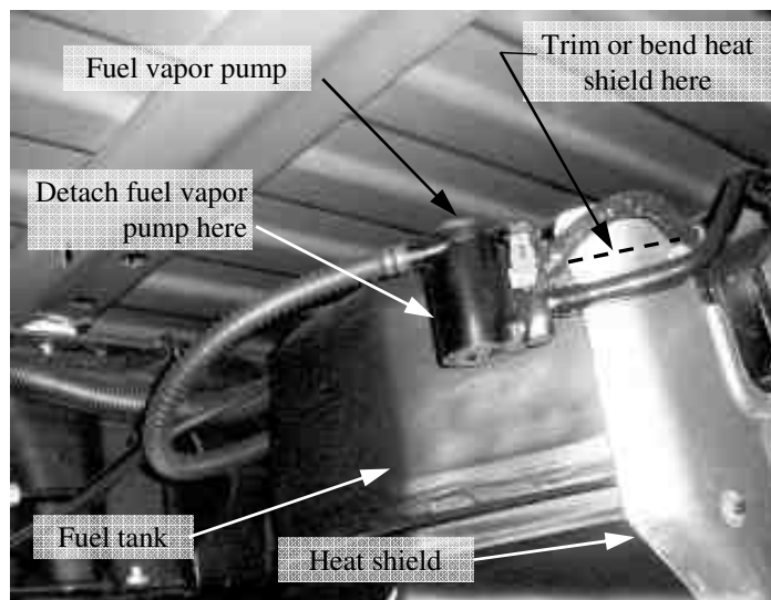
Figure 2 Rear of Gas Tank
